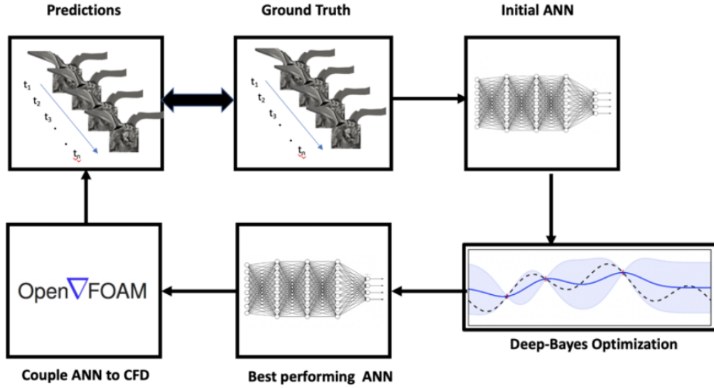
Figure 1: Schematic of the Bayesian Optimization based data-driven physical emulator workflow in identifying the best performing network hyper-parameters and network architecture
